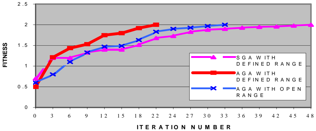
Figure (8): The best fitness plotted against the number of iterations for different learning.
