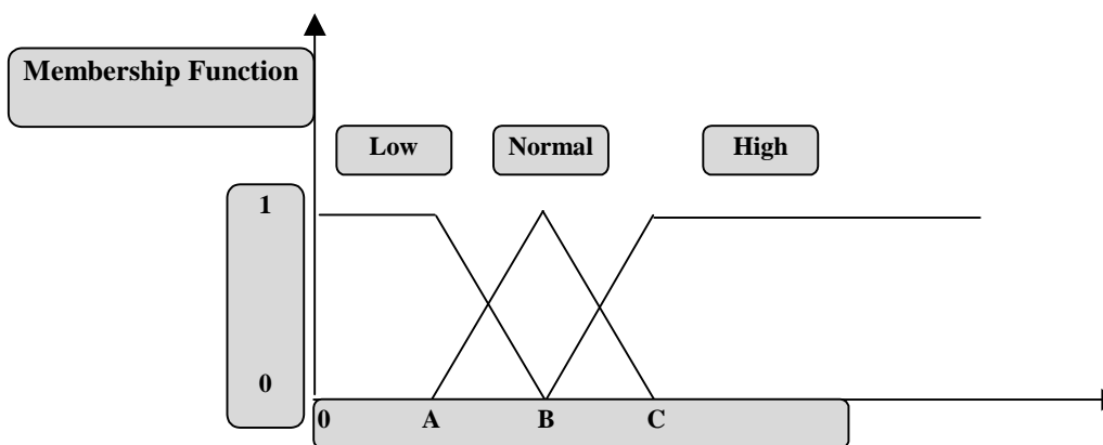
Figure (3): The input membership functions for RTEMP and ONTEMP A = 10^\circ , B = 20^\circ , C = 30^\circ , for RILLUM and ONILLUM A = 300 Lux, B = 400 Lux, C = 500 Lux.
