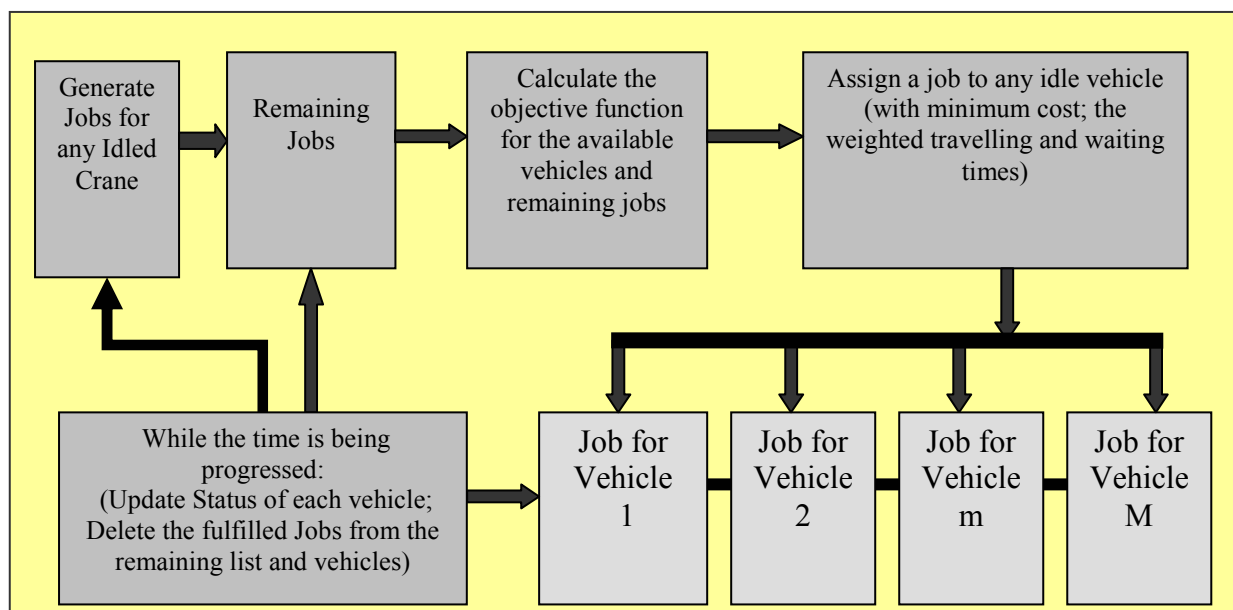
Figure 9: Block Diagram of the Greedy Heuristic Search in dynamic aspect
