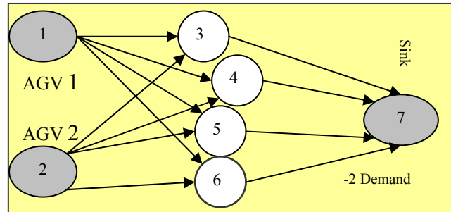
Figure 7: An example of network flow model for AGV scheduling.
