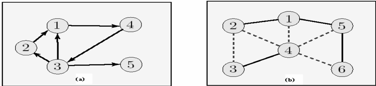
Figure 1: A connected Graph (a) and a spanning Tree (b) as dotted
