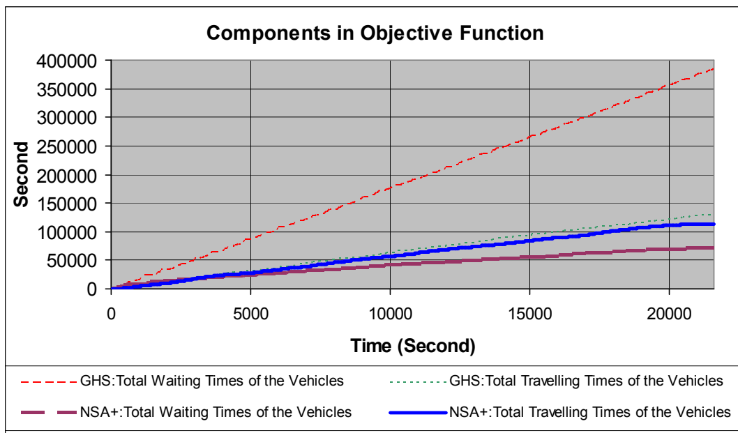
Figure 10: A comparison of Travelling and Waiting Times of the Vehicles
