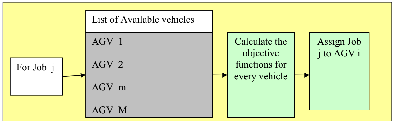
Figure 6: Block Diagram of Greedy Heuristic Search.
