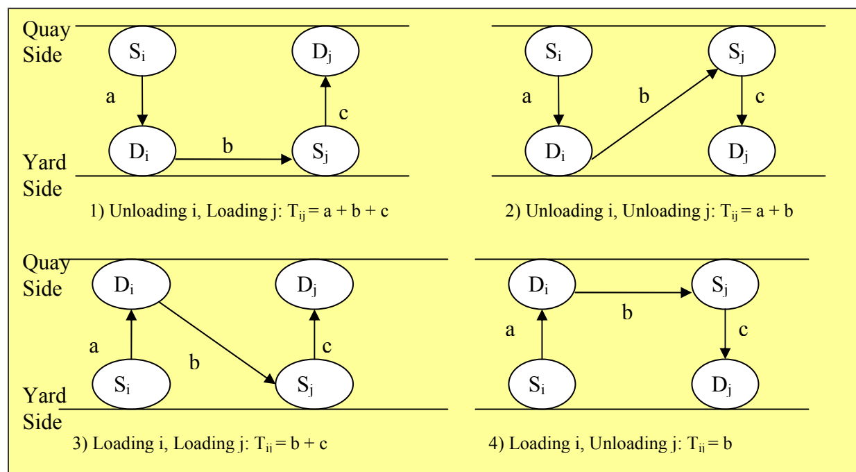
Figure 3: Travelling time computations between two jobs.
