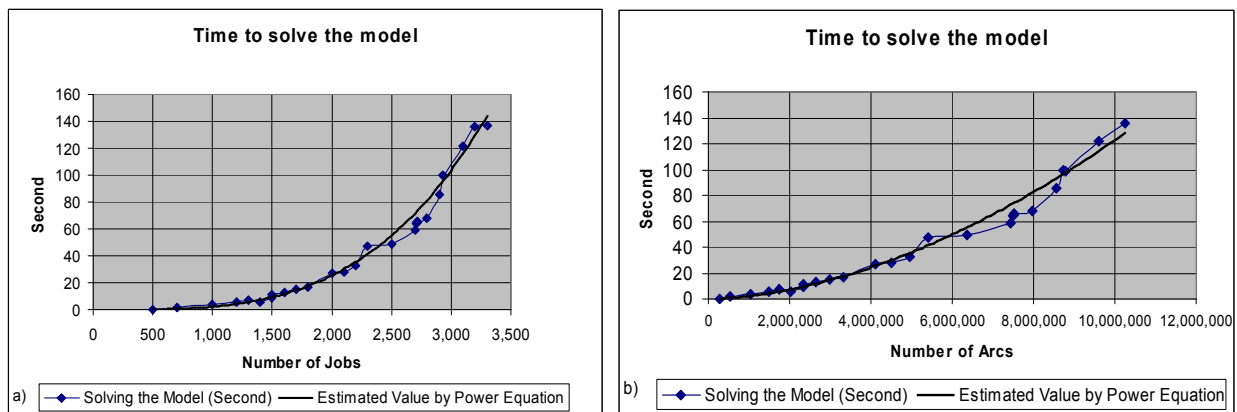
Figure 5: Time to solve the graph model (a) based on number of Jobs, b) based on number of Arcs
