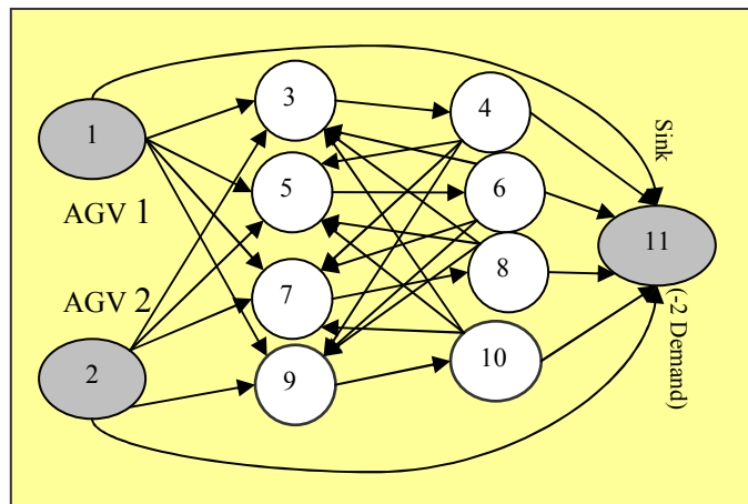
Figure 4: An example of network flow model for AGV scheduling.
