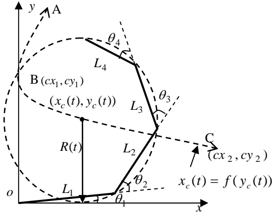
Fig. 5 The joint-end trajectory of C-shape fast turn
