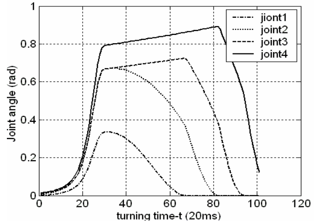
Fig. 7 The joint angle curves in a fast turn
