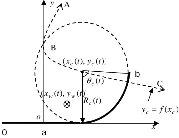
Fig. 9 Head-fixed relative coordinate system (HFRCS)
