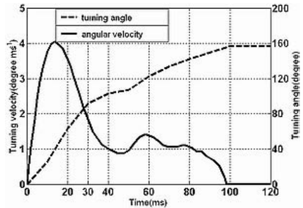
Fig. 12 The angular velocity and turning angle of a carp's C-shape sharp turn (recorded from [3])
