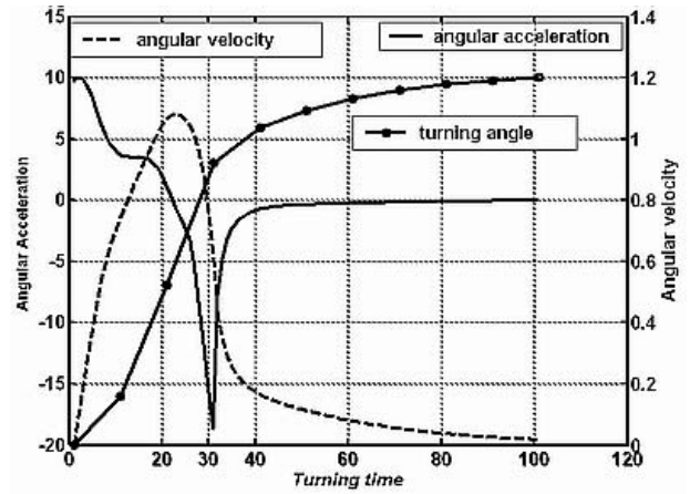
Fig. 11 Simulated angular acceleration, velocity and turning angle of C-shape sharp turn
