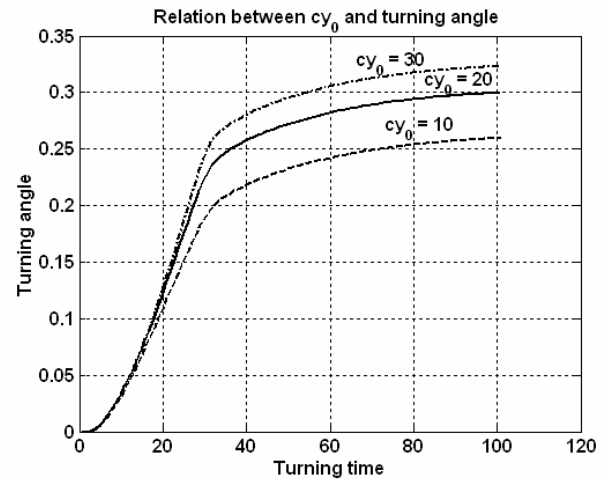
Fig. 13 The relation between cy_0 and turning angle
