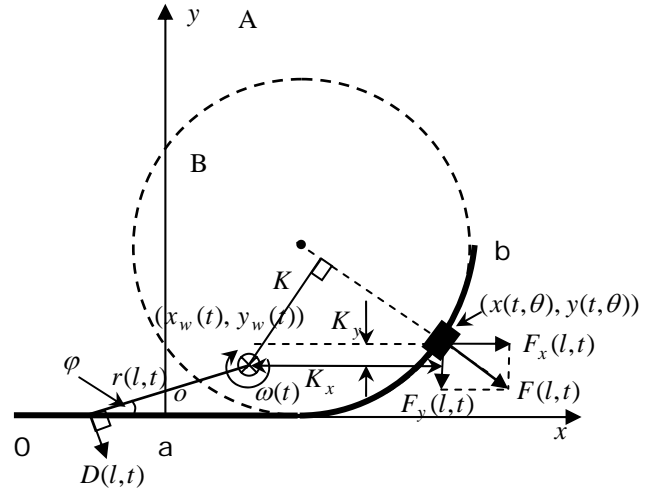
Fig. 10 Moment analysis of the robotic fish
