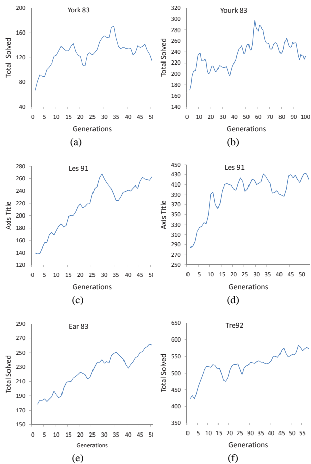
Fig. 4: The total number of individuals that have been able to generate a complete and valid timetable for the problem: (a) 500 individuals and 50 generations, (b) 500 individuals and 100 generations, (c) 500 individuals and 50 generations, (d) 1000 individuals and 50 generations, (e) 500 individuals and 50 generations, (f) 1000 individuals and 60 generations.
