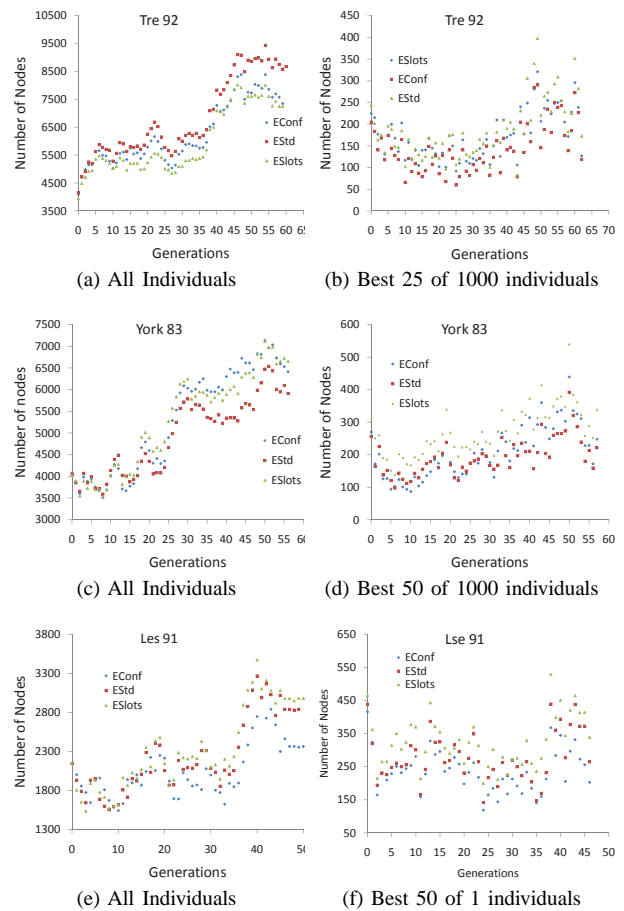
Fig. 5: The total number of the exam selection grammar components in each generation, the data in the graphs on the left hand side is collected from all individuals exist in each generation, in (b) the data is collected from the best 25 individuals out of 1000 shown in (a), in (d) the data is collected from the best 50 individuals out of 1000 shown in (c), in (f) the data is collected from the best 25 individuals out of 1000 shown in (e).
