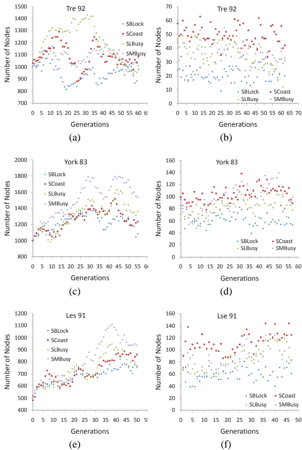
Fig. 6: The total number of the slot selection heuristics in each generation, the data in the graphs on the left side is collected from all individuals exist in each generation, in (b) the data is collected from the best 25 individuals out of 1000 shown in (a), in (d) the data is collected from the best 50 individuals out of 1000 shown in (c), in (f) the data is collected from the best 25 individuals out of 1000 shown in (e).
